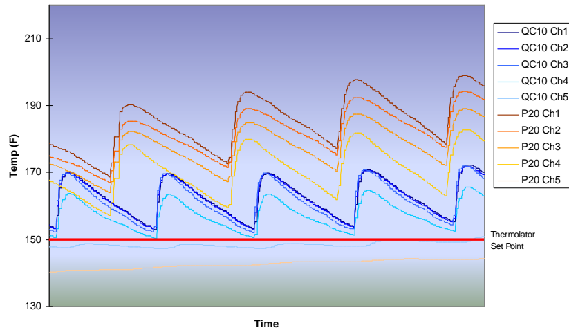
Nylon, 555 Melt Temp, 90 Sec
