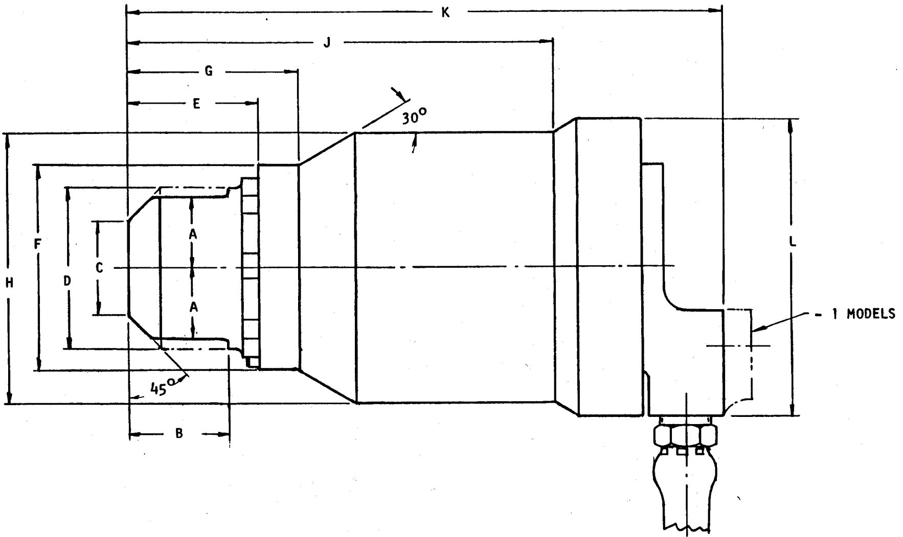
CLEARANCE DIMENSIONS
