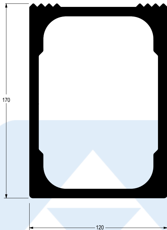
CA-0353 14,329 kg/m Barrote
