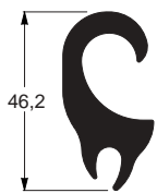
EE-1783 1,268 kg/m
