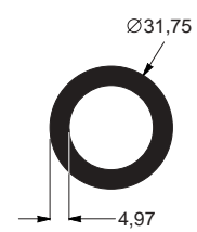
TR-1088 1,134 kg/m Tubo redondo
