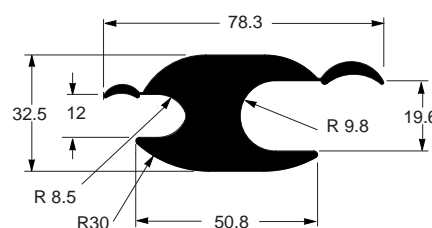
EE-0715 2,771 kg/m Conector
