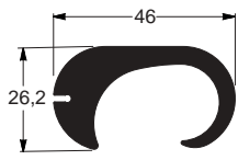
EE-0677 1,311 kg/m
