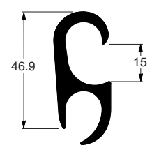
EE-0647 1,198 kg/m Corpo conector
