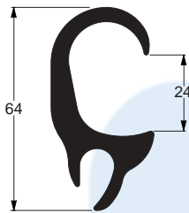
EE-1782 1,770 kg/m
