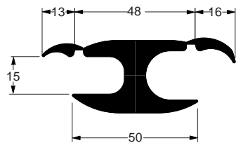
EE-0769 2,369 kg/m Had 300 a 400 conector
