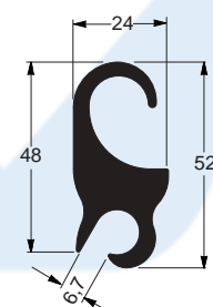
EE-0638 1,485 kg/m
