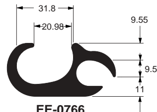
EE-0766 1,929 kg/m Conector
