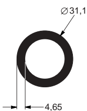
TR-1081 1,047 kg/m Tubo redondo
