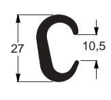
EE-1784 0,489 kg/m Conector
