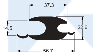
EE-0719 1,427 kg/m Conector
