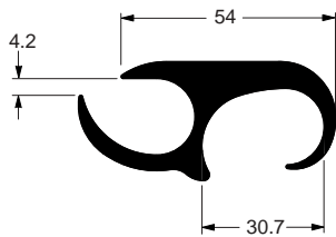
EE-0771 1,728 kg/m Conector
