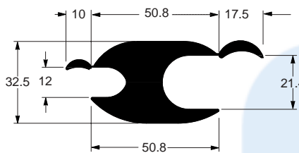
EE-0760 2,676 kg/m Had 50066
