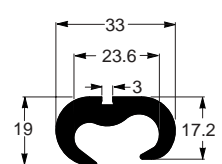
EE-0636 0,779 kg/m Conector
