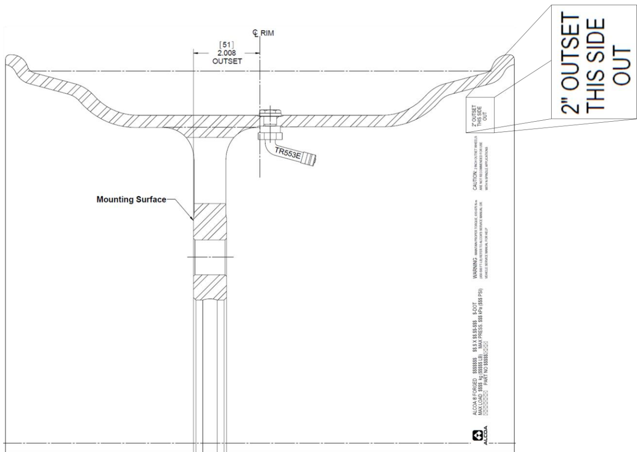
Figure 3 - (2” Outset)
