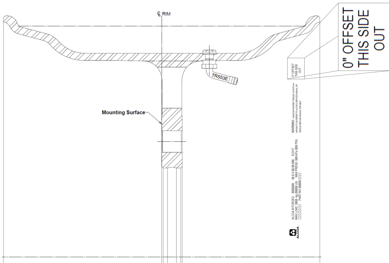
Figure 1 - (0” Offset)
